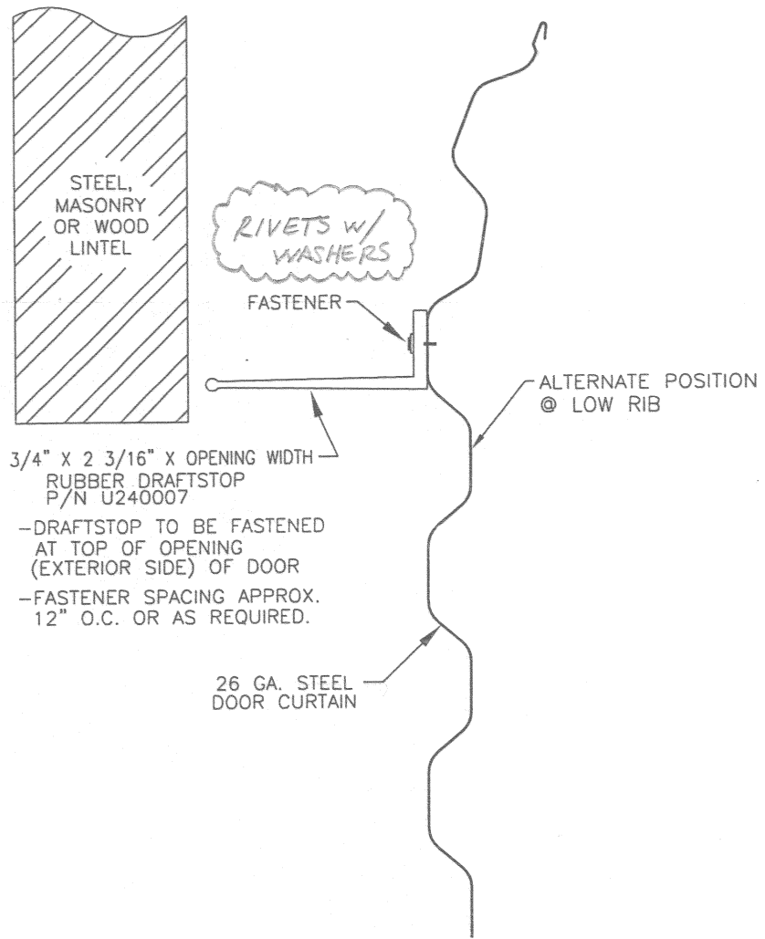
(A) DETAIL AT DOOR HEAD N.T.S.
